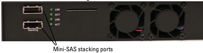
Figure 1-6. N2048 Mini-SAS Stacking Ports and Fans
